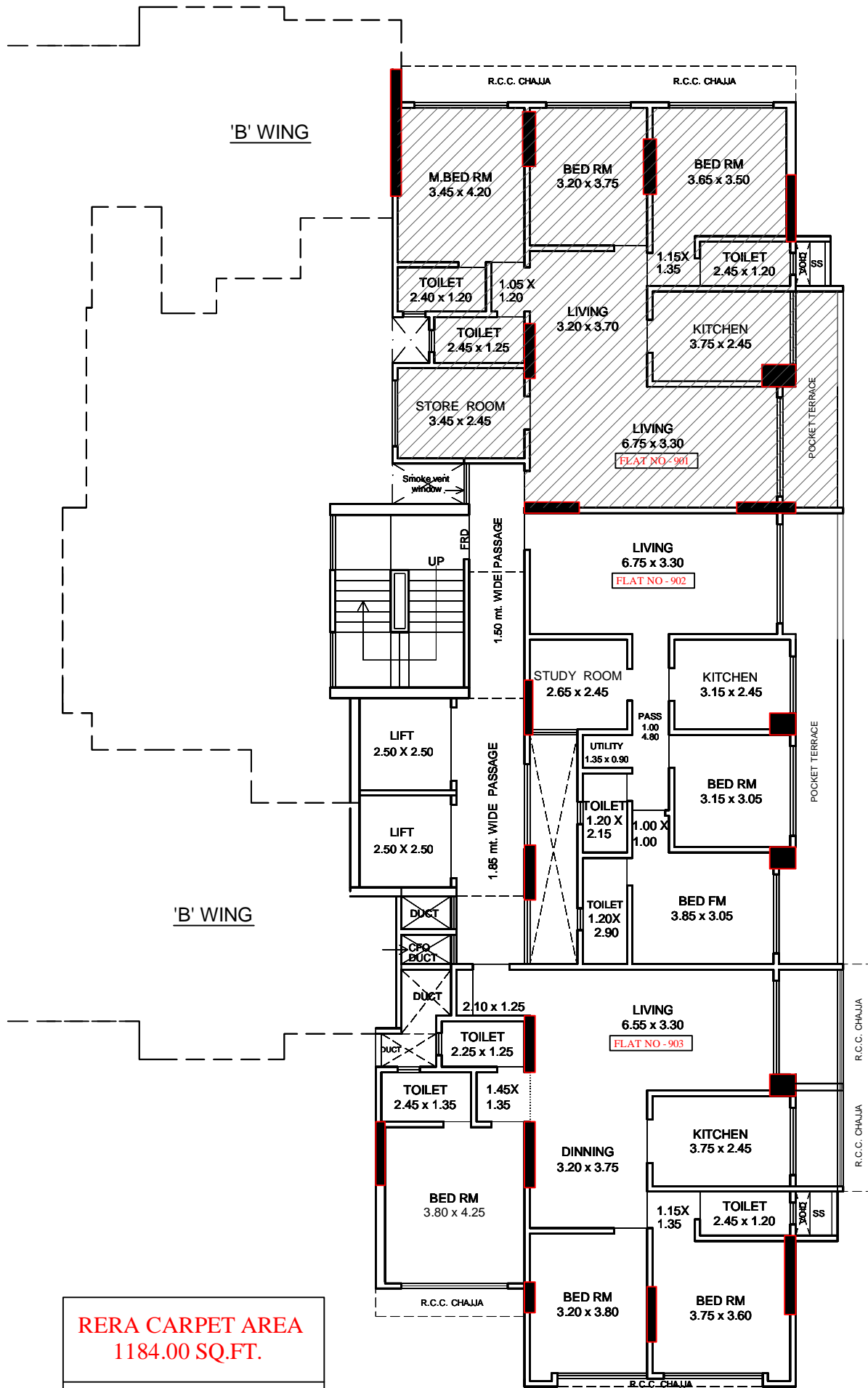
9TH FLOOR PLAN 'A' WING
