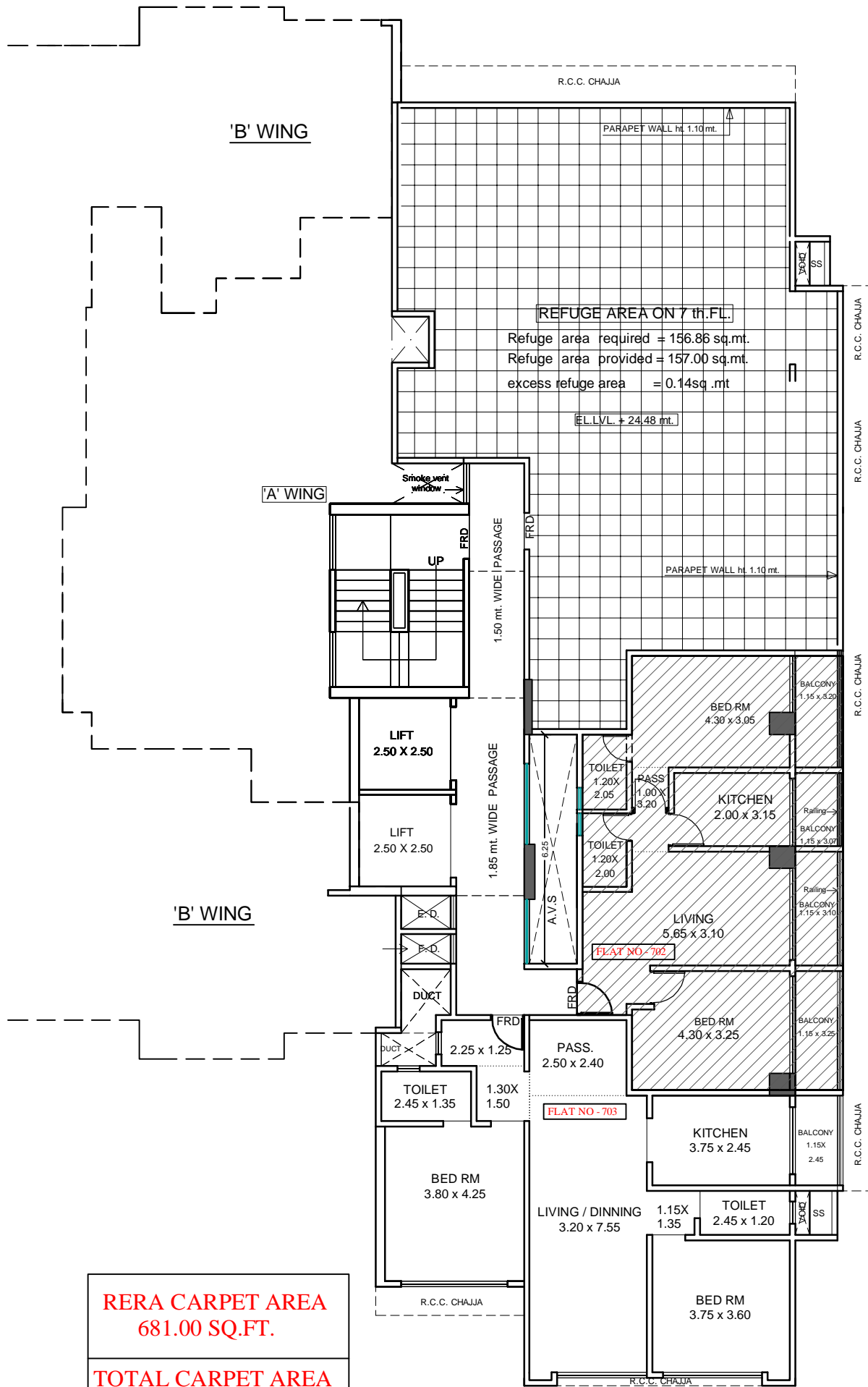
7TH FLOOR PLAN 'A' WING
