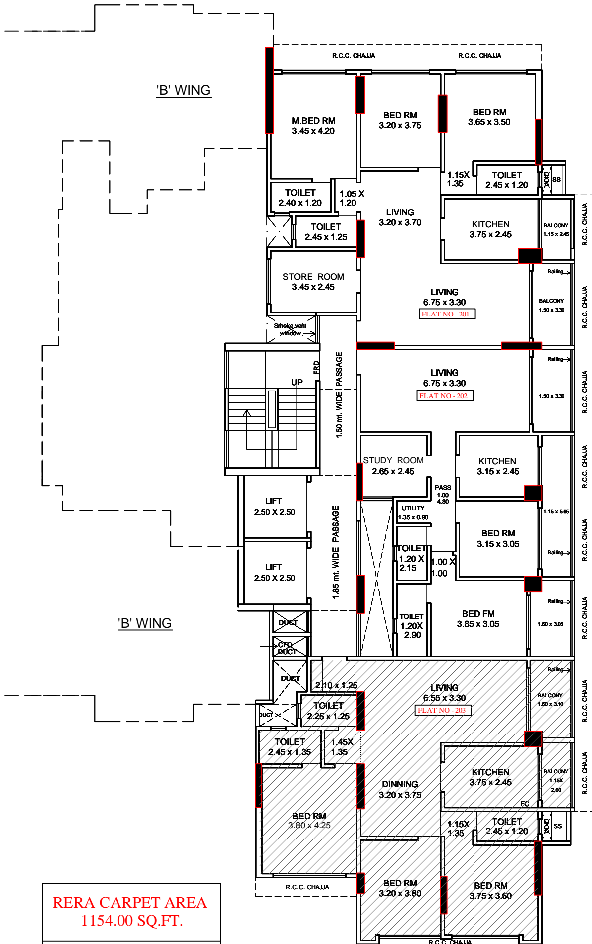
2ND FLOOR PLAN 'A' WING
