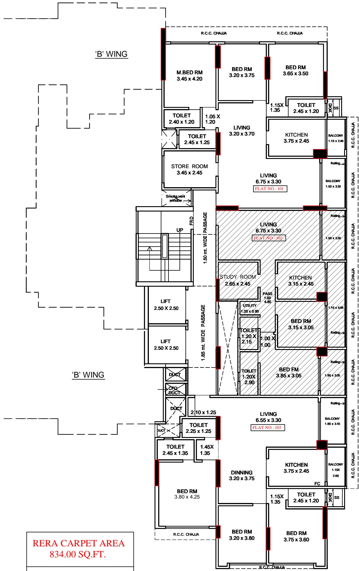
1ST FLOOR PLAN 'A' WING
